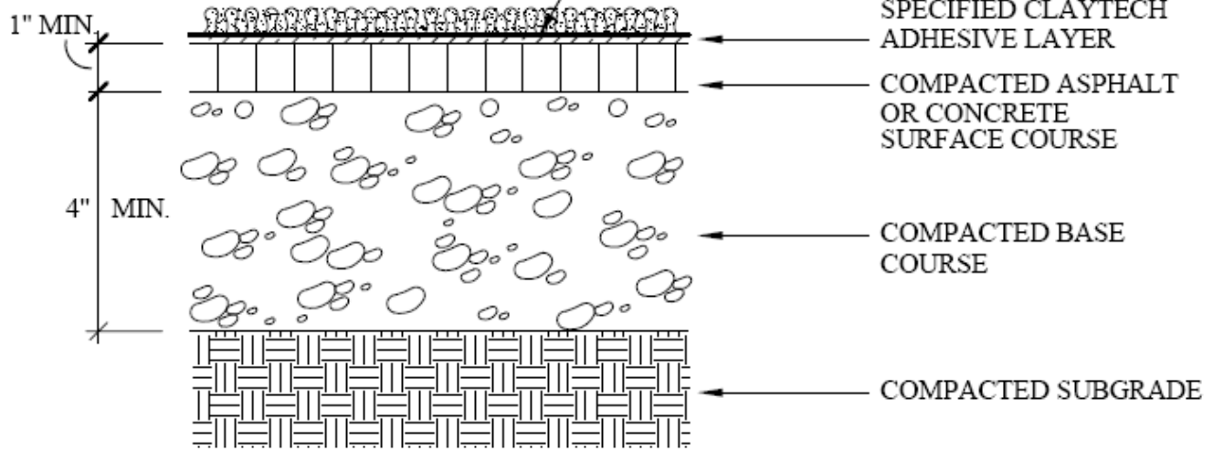
FOR NEW COURT IN NON FREEZE/THAW CLIMATE
