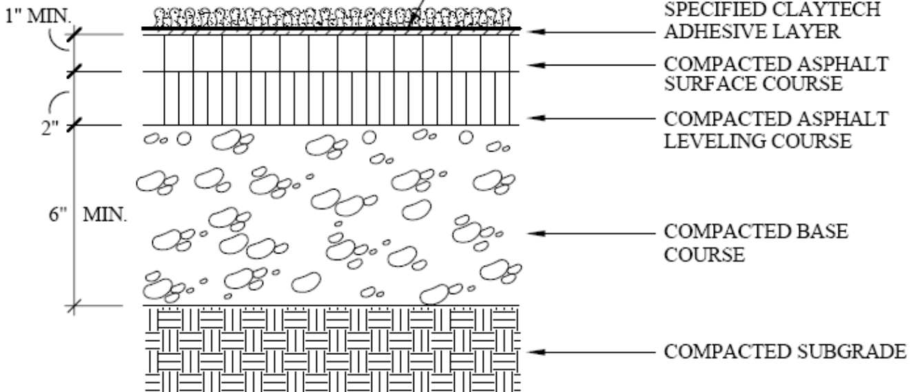
FOR NEW ASPHALT COURT IN FREEZE/THAW CLIMATE
